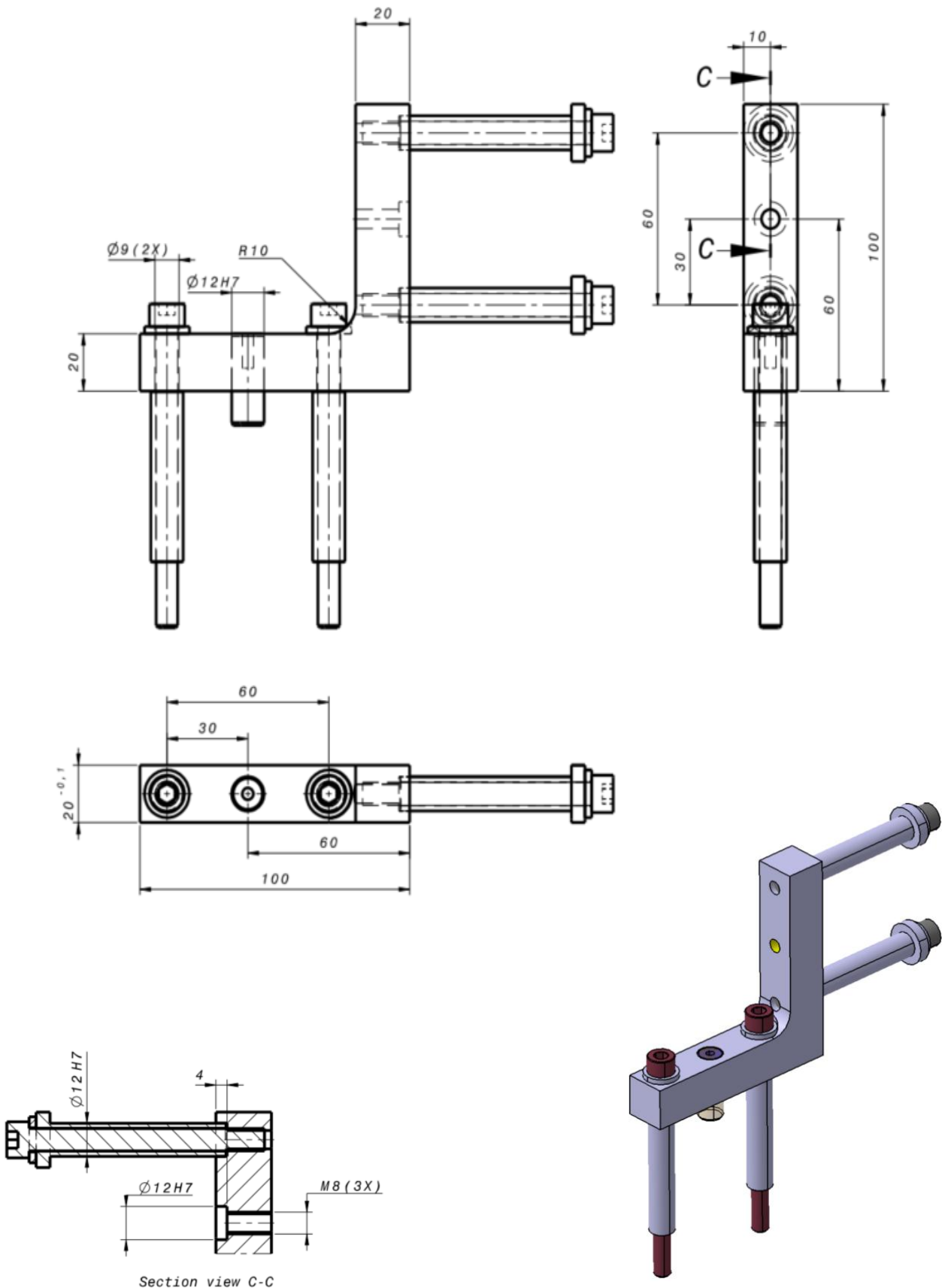
Section view C-C
